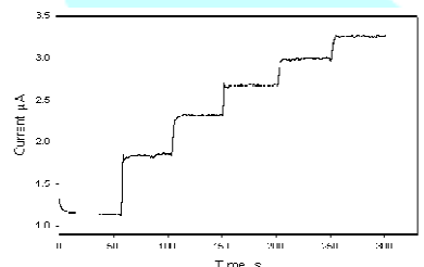
Typical response of the biosensor toward the sequential injection of 0.02 mM H_2O_2 at -100 mV vs. Ag/AgCl. The biosensor was prepared with 1.0 mg mL^{-1} CNTs and 7 electropolymerization cycles of PANI.
